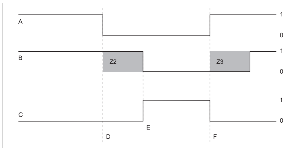
Fig. 25: Alarm signalling and dosing switch-off by the main stream
