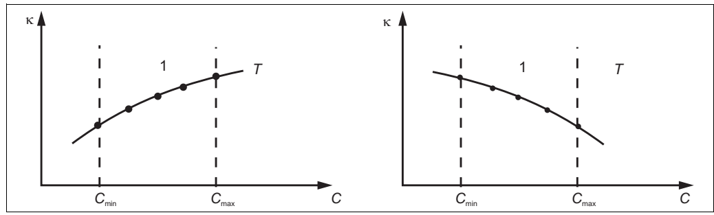
Fig. 36: Measured data for a constant process temperature (example) κ Conductivity C Concentration T Constant temperature 1 Measuring range
