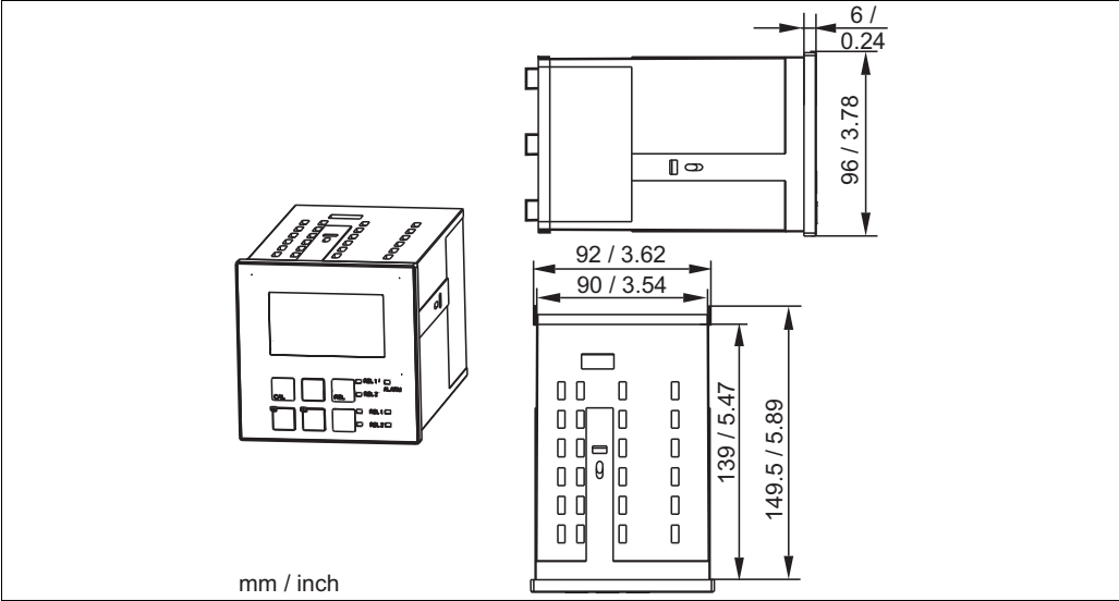
Fig. 4: Panel-mounted instrument
