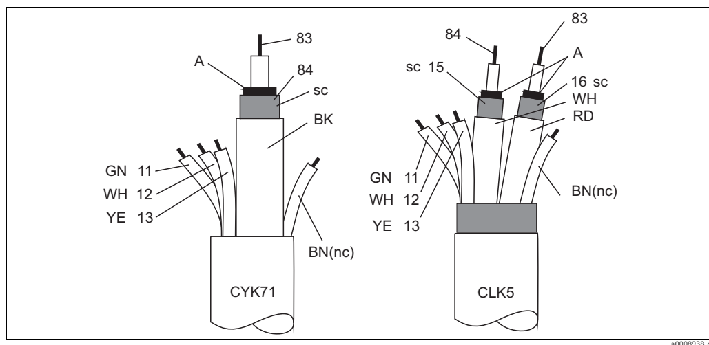
Fig. 12: Structure of the special measuring cables
