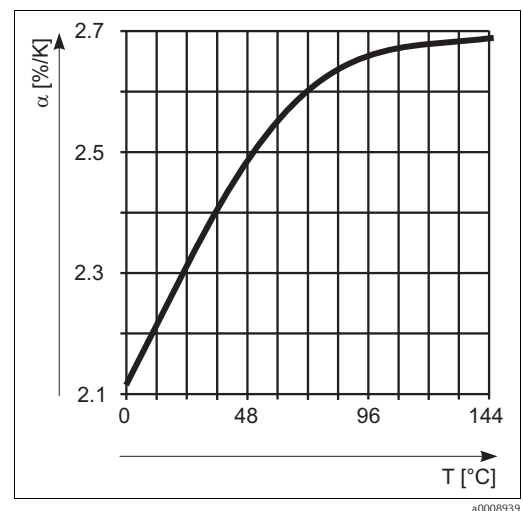
Fig. 23: NaCl compensation
