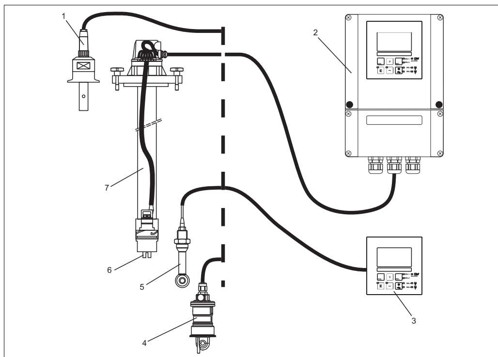
Fig. 1: Complete measuring system Liquisys M CLM223/253
