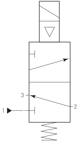
FIGURE 1 - SPRING RETURN VALVE 3/2 WAY
