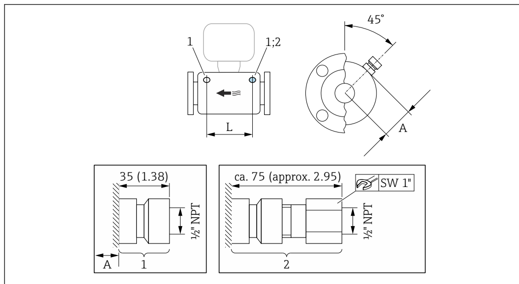
34 Engineering unit mm (in)
