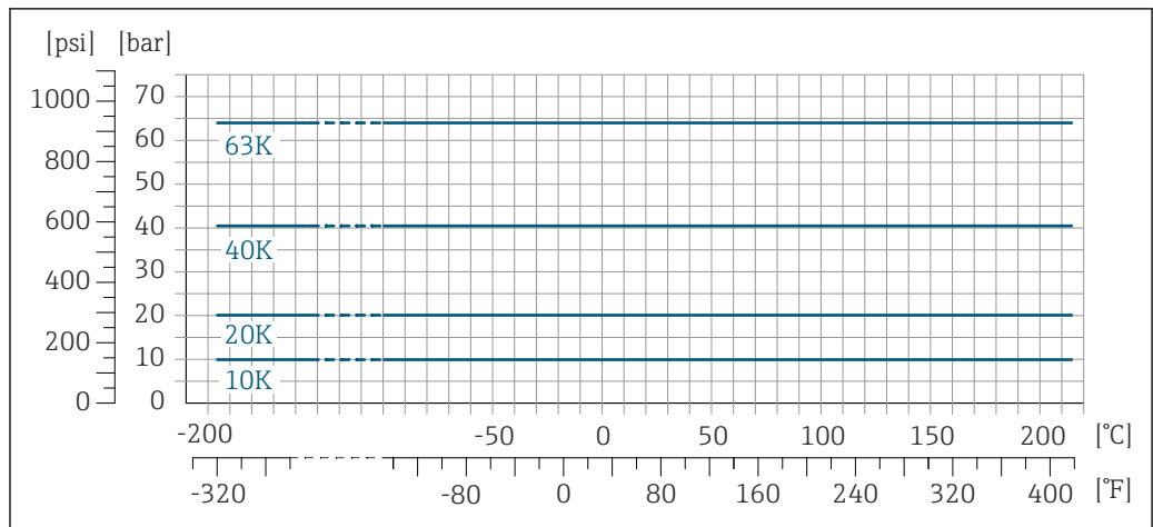
27 With flange material 1.4404 (F316/F316L)
