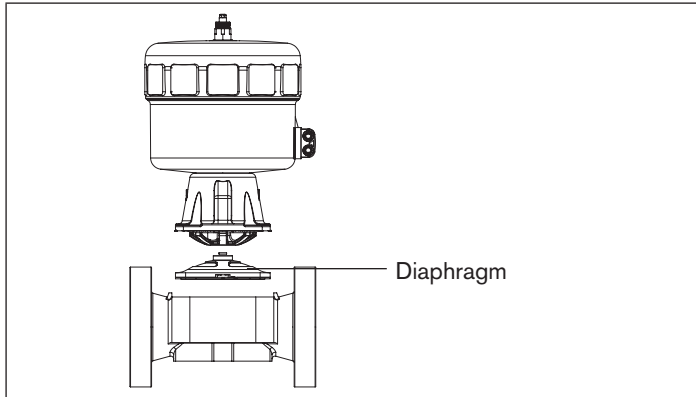
Fig. 16: Diaphragm replacement part
