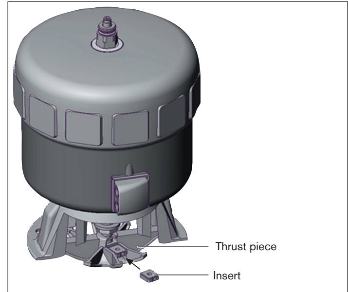
Fig. 13: Installation of the insert
