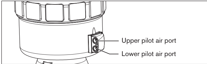
Fig. 12: Pilot air port
