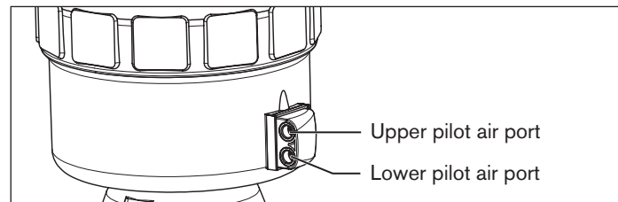
Fig. 14: Pneumatic connection
