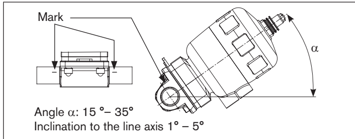
Fig. 9: Installation position for self-drainage of the body
