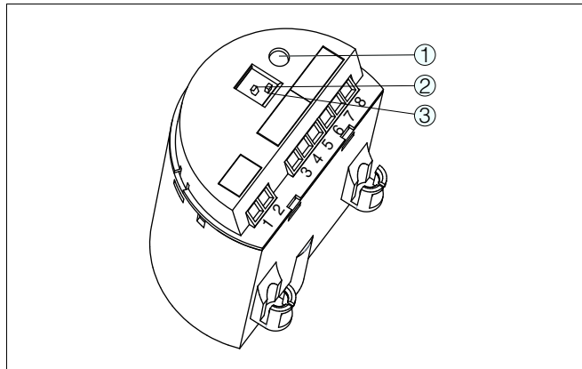
Fig. 12: Oscillator SWE60R - Relay output
