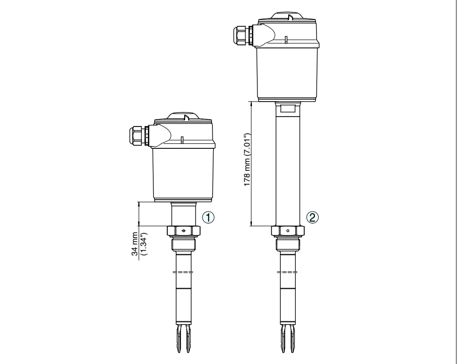
Fig. 34: Options Gas-tight leadthrough Temperature adapter
