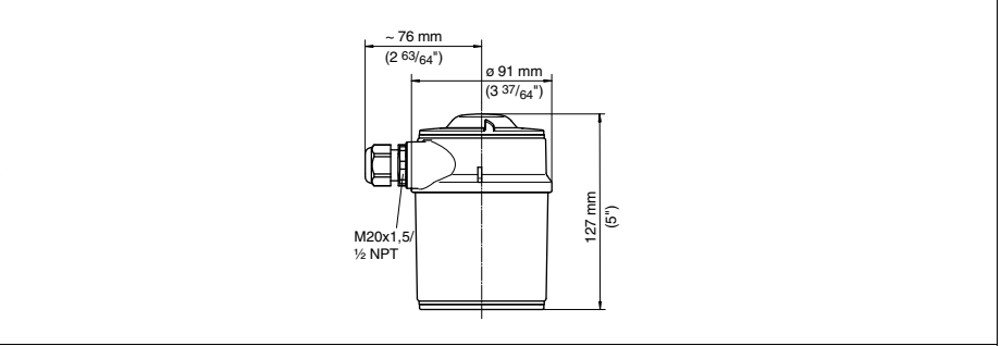
Fig. 32: Housing
