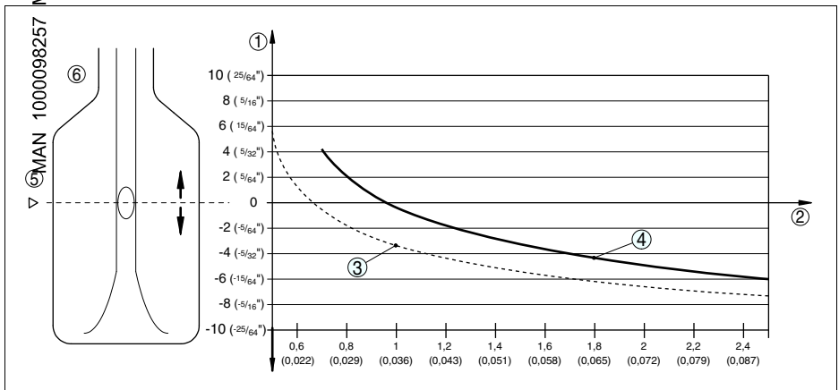
Fig. 27: Influence of the product density on the switching point
