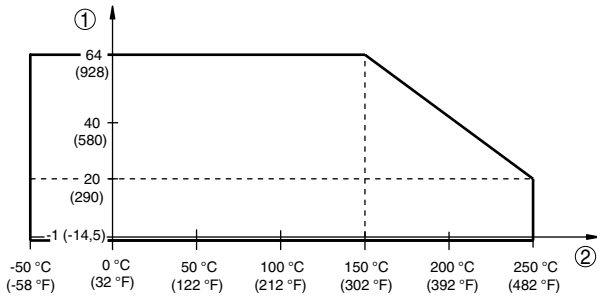
Fig. 31: Process temperature - Process pressure with switch position 0.5 g/cm 3 (sensitivity switch) Process pressure in bar (psig) Process temperature in °C (°F)
