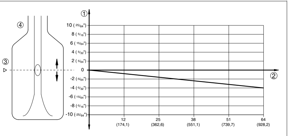
Fig. 28: Influence of the process pressure to the switching point
