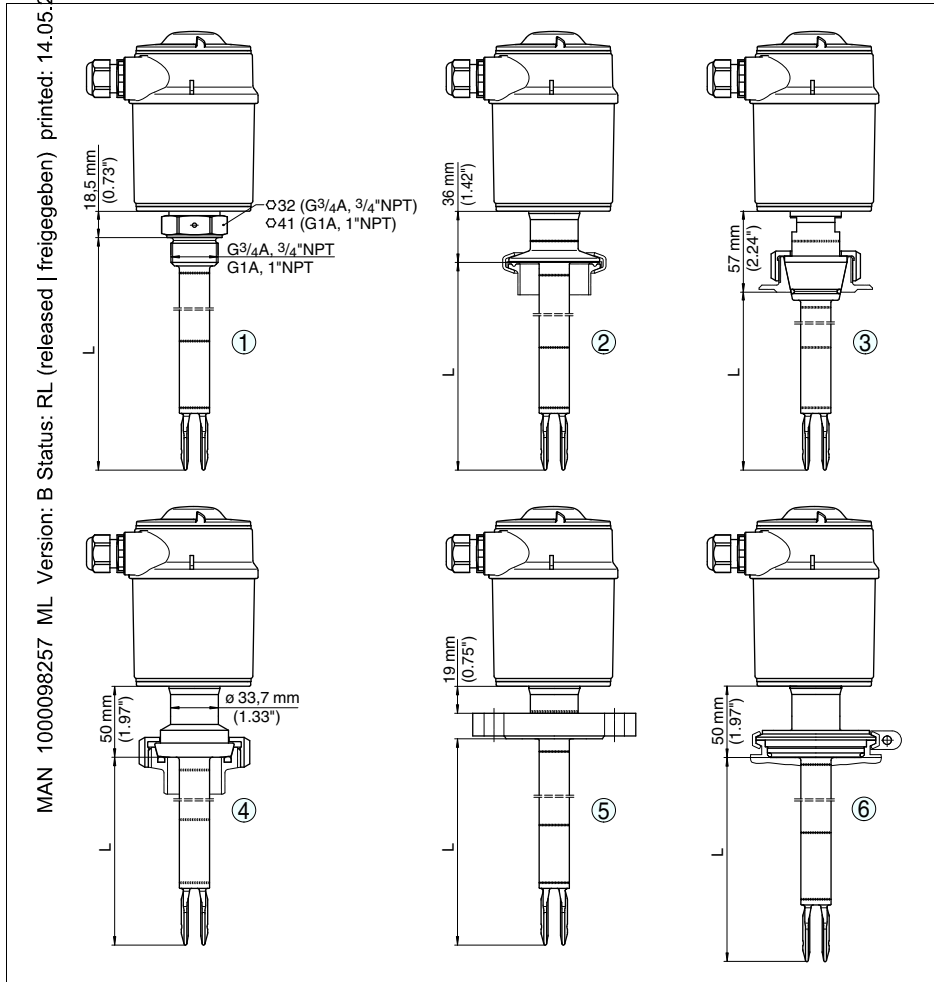
Fig. 36: LEVEL SWITCH 8112
