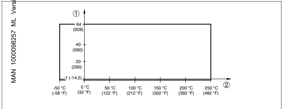
Fig. 30: Process temperature - Process pressure with switch position 0.7 g/cm 3 (sensitivity switch)
