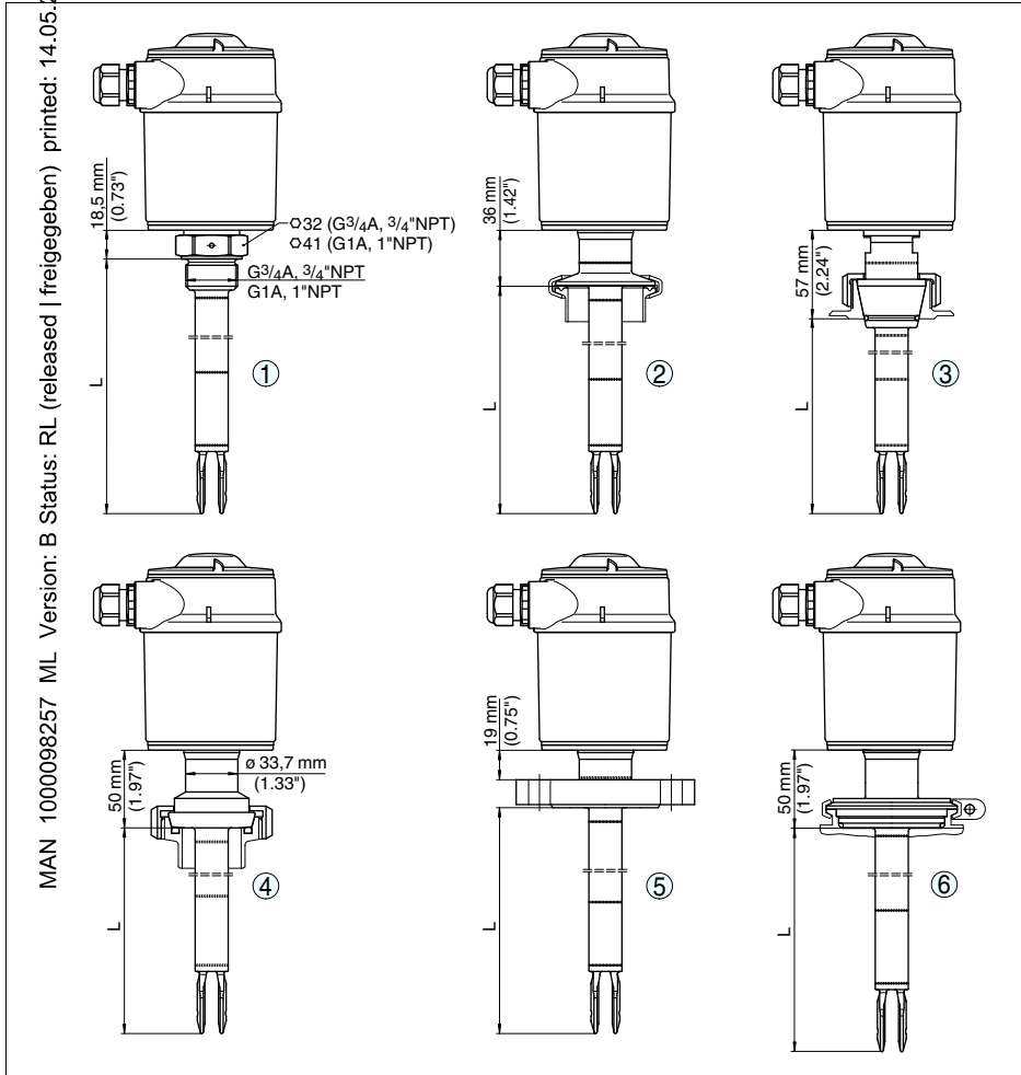
Fig. 33: LEVEL SWITCH 8112
