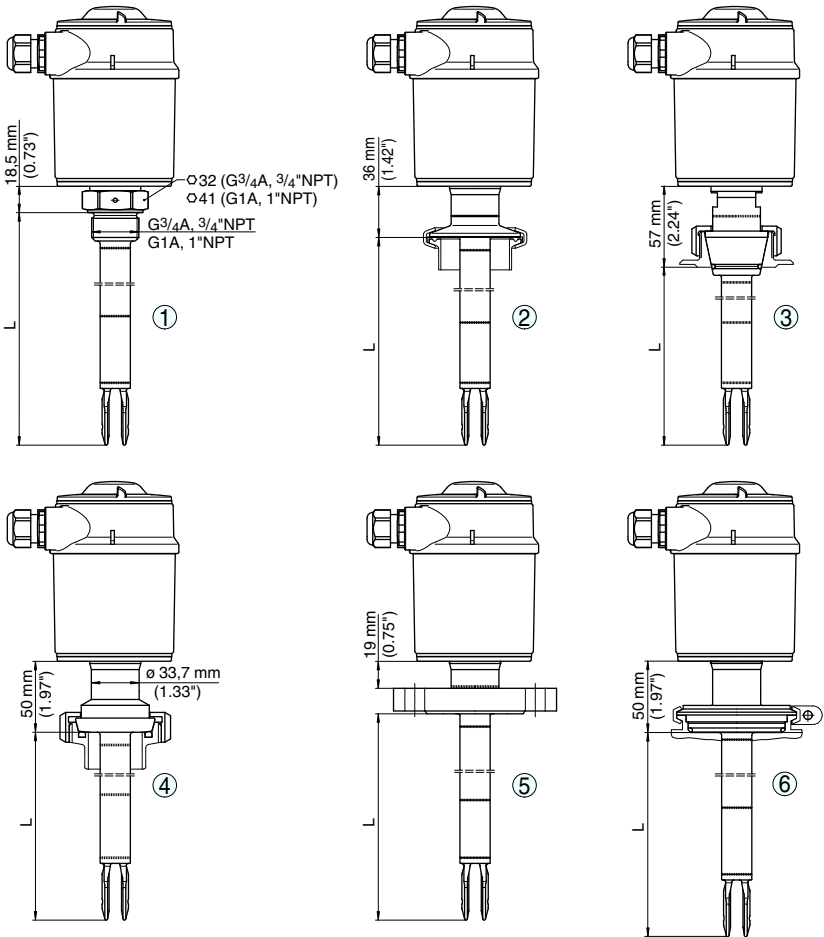
Abb. 33: LEVEL SWITCH 8112
