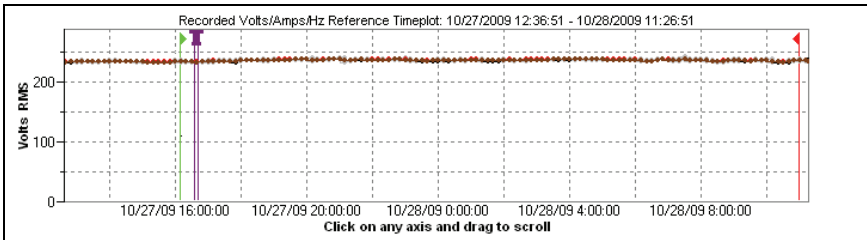
Figure 11. Annotation View
