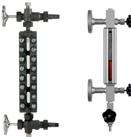
Sight glass level indicator, model LGG, examples
