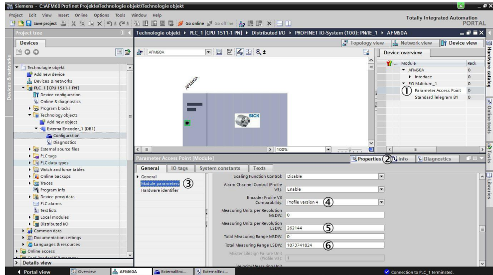
Figure 26: Device view
