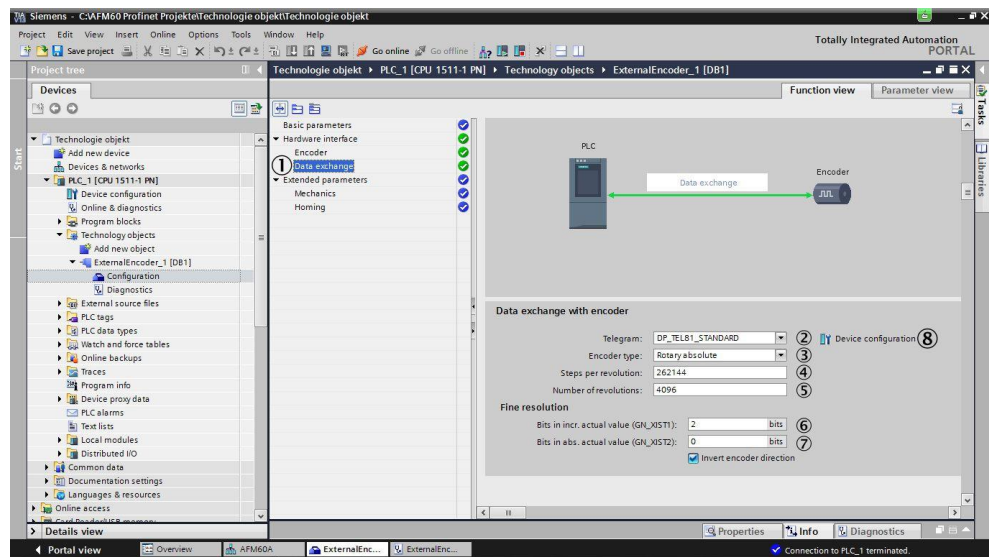
Figure 25: Data exchange
