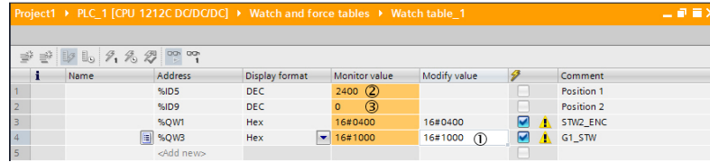
Figure 18: Setting bit 12 of G1_STW
