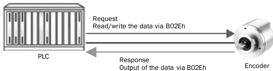
Figure 5: Request and Response
