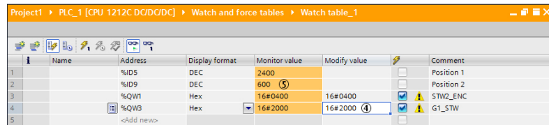
Figure 19: Setting bit 13 of G1_STW
