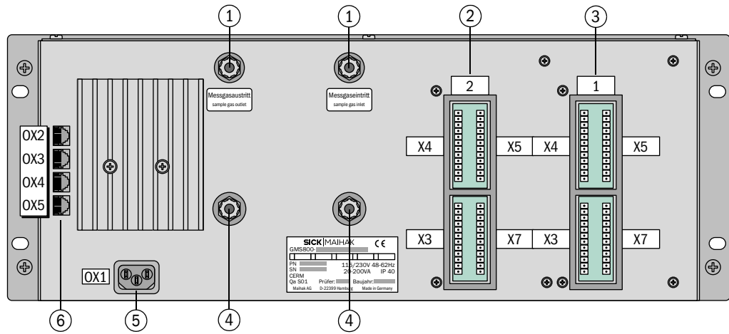
Fig. 1 Connections
