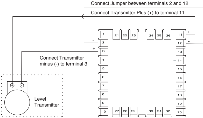
Figure 3 - Transmitter Wiring
